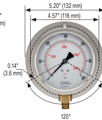
40-901 Rear Flange
