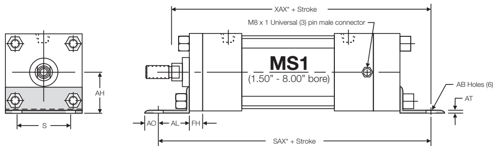
'MS1' PFLF Cylinder Dimensions - Standard Rod Only
