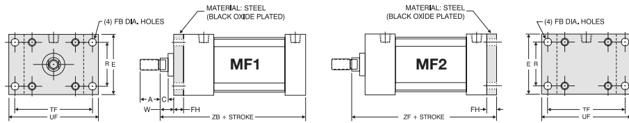
'FM' Series 'MF1' and 'MF2' Flange Mount Dimensions
