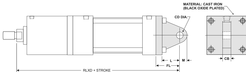
'FM' Series 'MP4' Rod Eye Mount Dimensions
