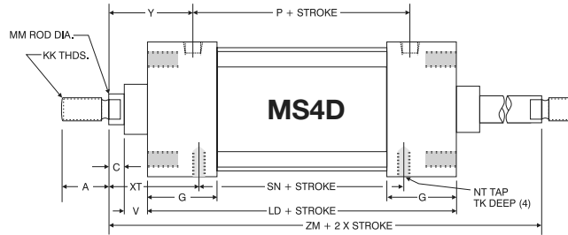
'FM' Series Double Rod End 'MS4D' Flush Mount Dimensions
