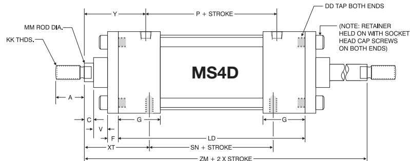
'FM' Series Double Rod End Oversize Rod 'MS4D' Flush Mount Dimensions
