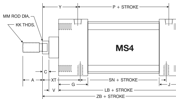
'FM' Series Oversize Rod 'MS4' Flush Mount Dimensions
