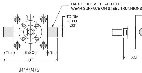
'FM' Series 'MT1' Head Trunnion and 'MT2' Cap Trunnion Mount Dimensions
